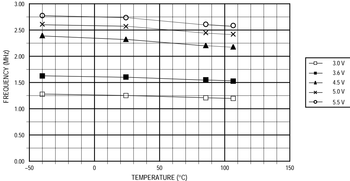
Figure C-3. Typical Internal Operating Frequency versus Temperature (OSCREG Bit = 1)
